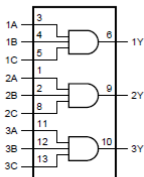
Figure 1. Functional diagram
